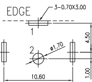
PCB LAYOUT (BOTTOM VIEW)
