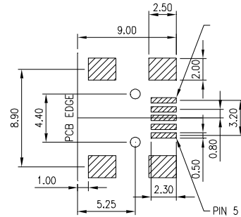
RECOMMENDED PCB PATTERN LAYOUT (PCB THICKNESS:0.8±0.1)
