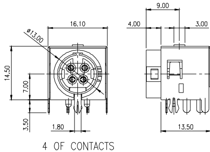
4 OF CONTACTS
