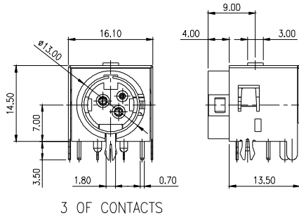
3 OF CONTACTS
