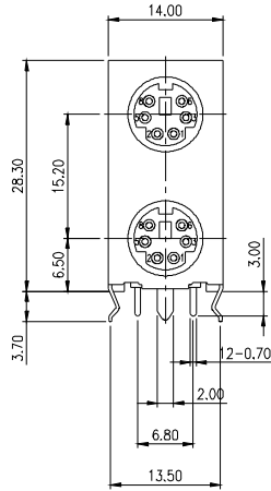
STANDARD TYPE 12 OF CONTACTS
