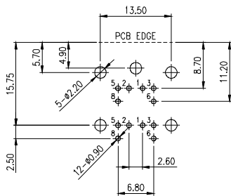
WITH GROUNDING SPRING 12 OF CONTACTS
