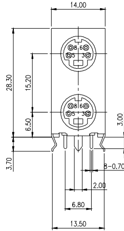
STANDARD TYPE 8 OF CONTACTS
