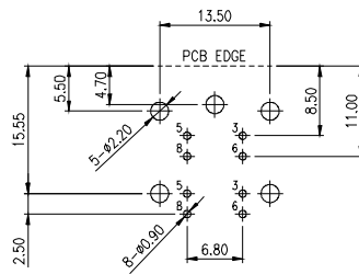
STANDARD TYPE 8 OF CONTACTS
