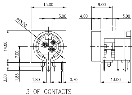
3 OF CONTACTS
