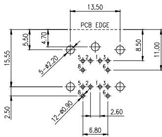
STANDARD TYPE 12 OF CONTACTS
