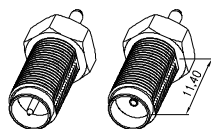
20: SMA JACK 11.4mm (FEMALE)
