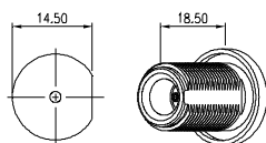
40: N JACK 1-FLAT 18.5mm BLK (FEMALE)
