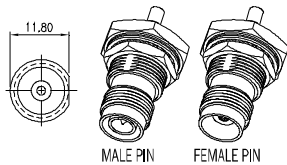
10: TNC JACK 1-FLAT (FEMALE)
