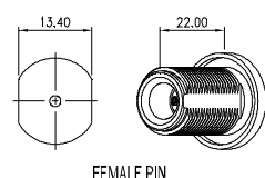
41a: N JACK 2-FLAT 22.0mm BLK (FEMALE)
