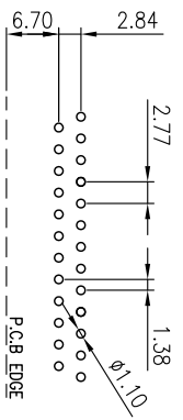
RECOMMENDED P.C.B LAYOUT
